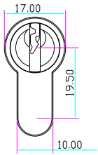
Single side cylinde
